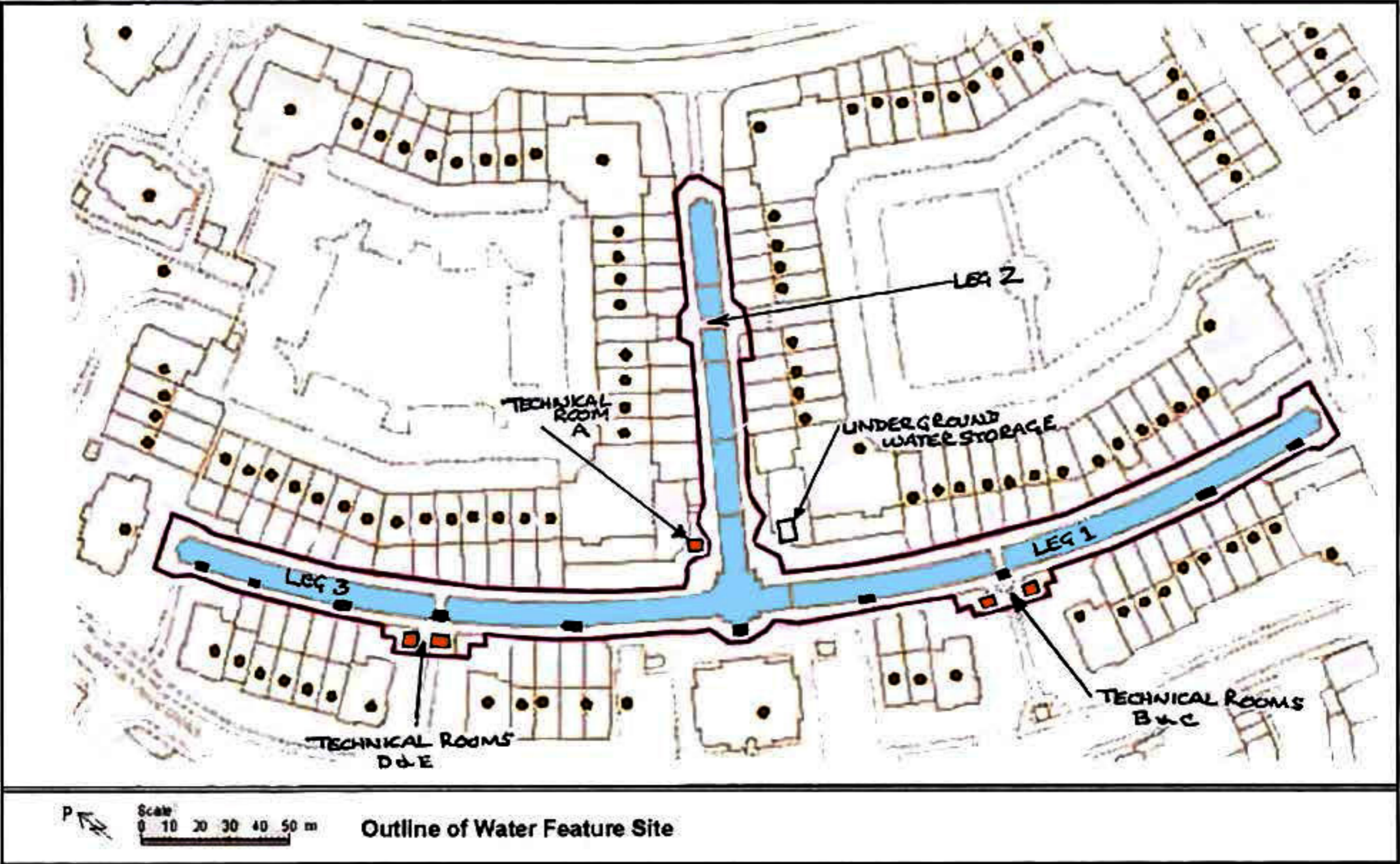
Extent of Water Feature showing location of Pump Chambers ■ and Technical Rooms ABCDE
